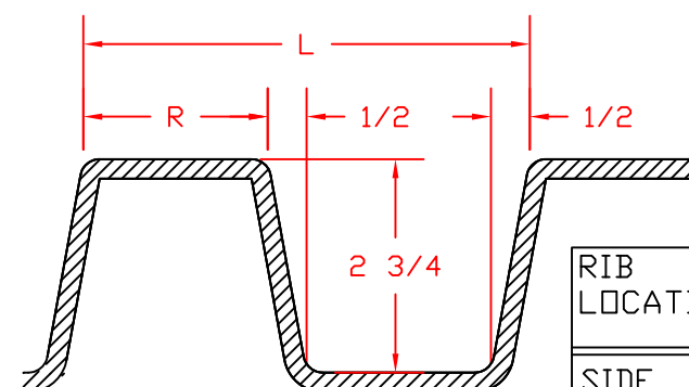
RIB DETAIL 1/2 SCALE
