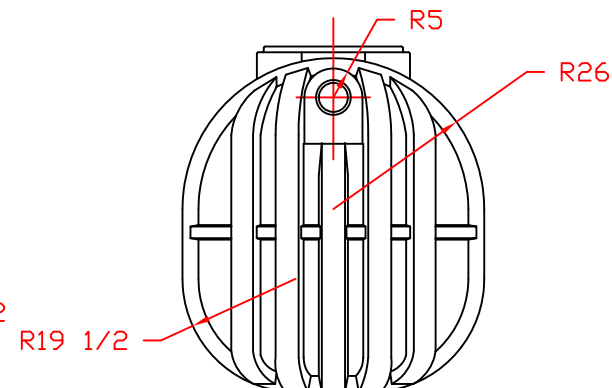
RIB DETAIL 1/2 SCALE
